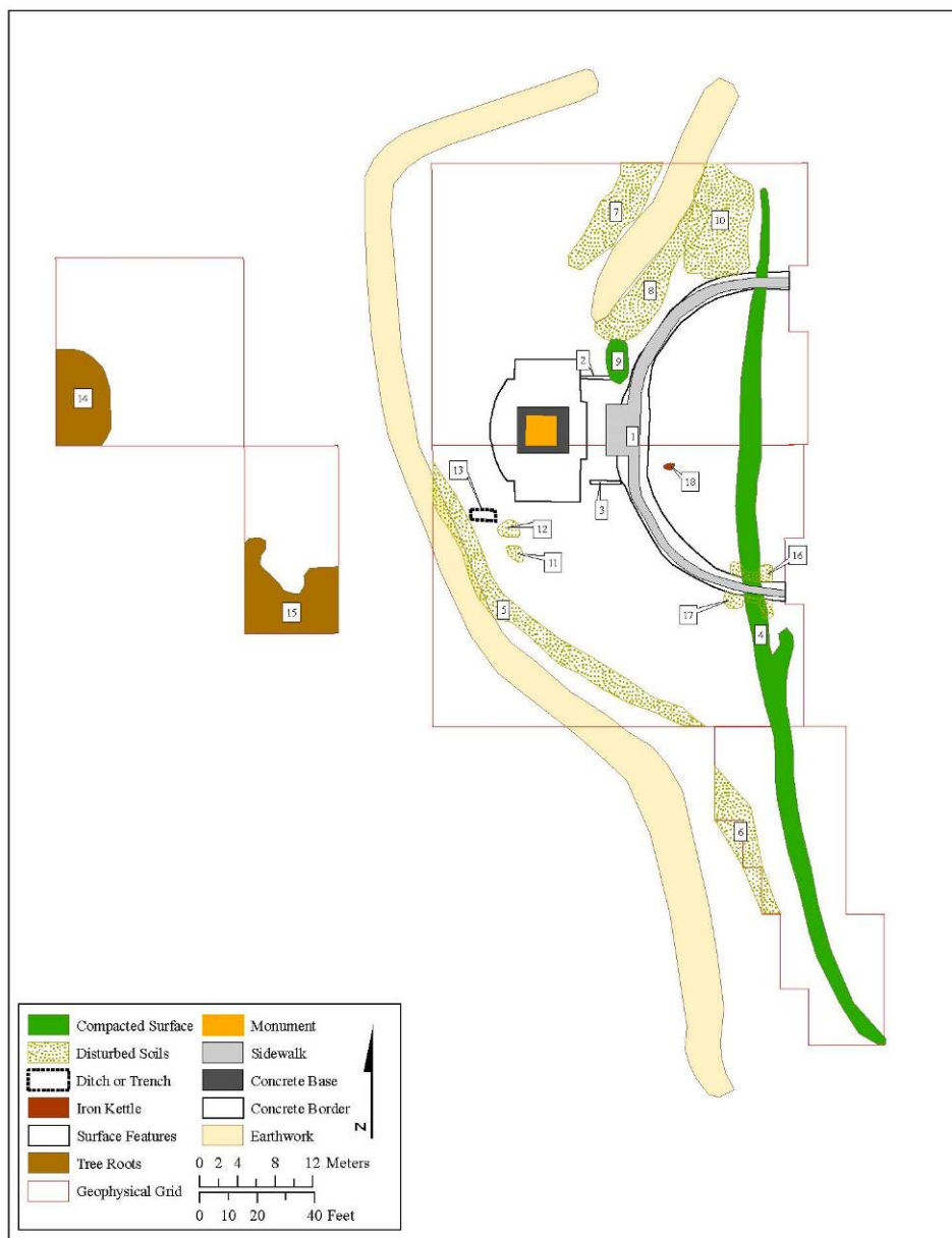
FIGURE 16. Interpretation of ground penetrating radar survey.
