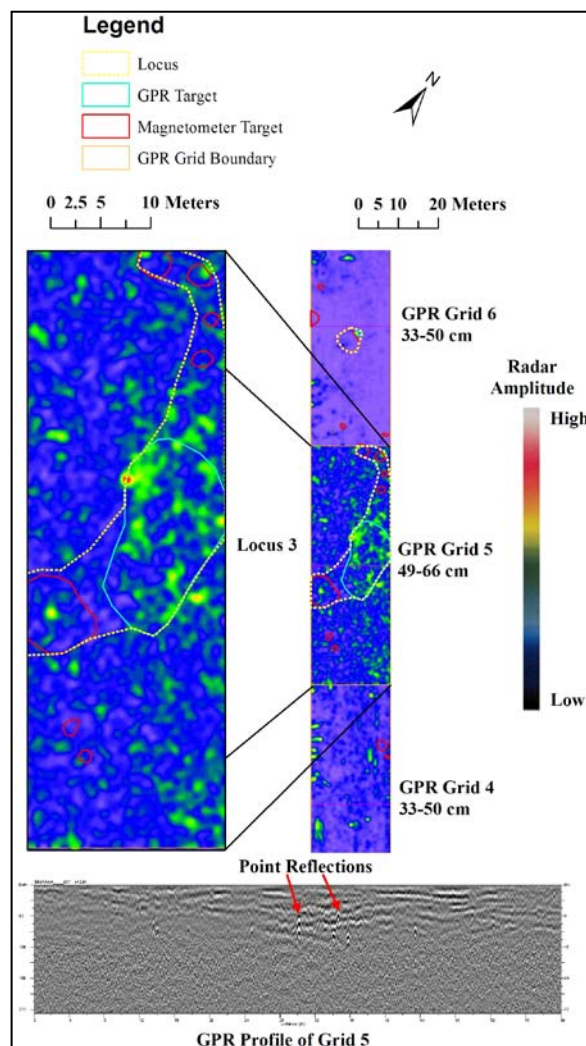
FIGURE 9. GPR results.
