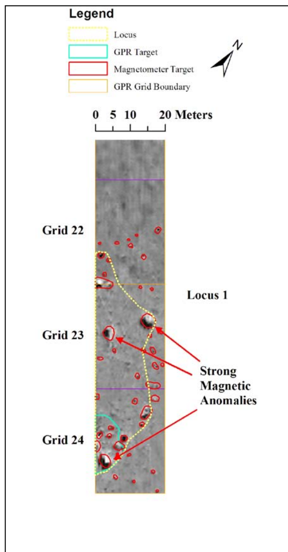
FIGURE 8. Magnetometer results.
