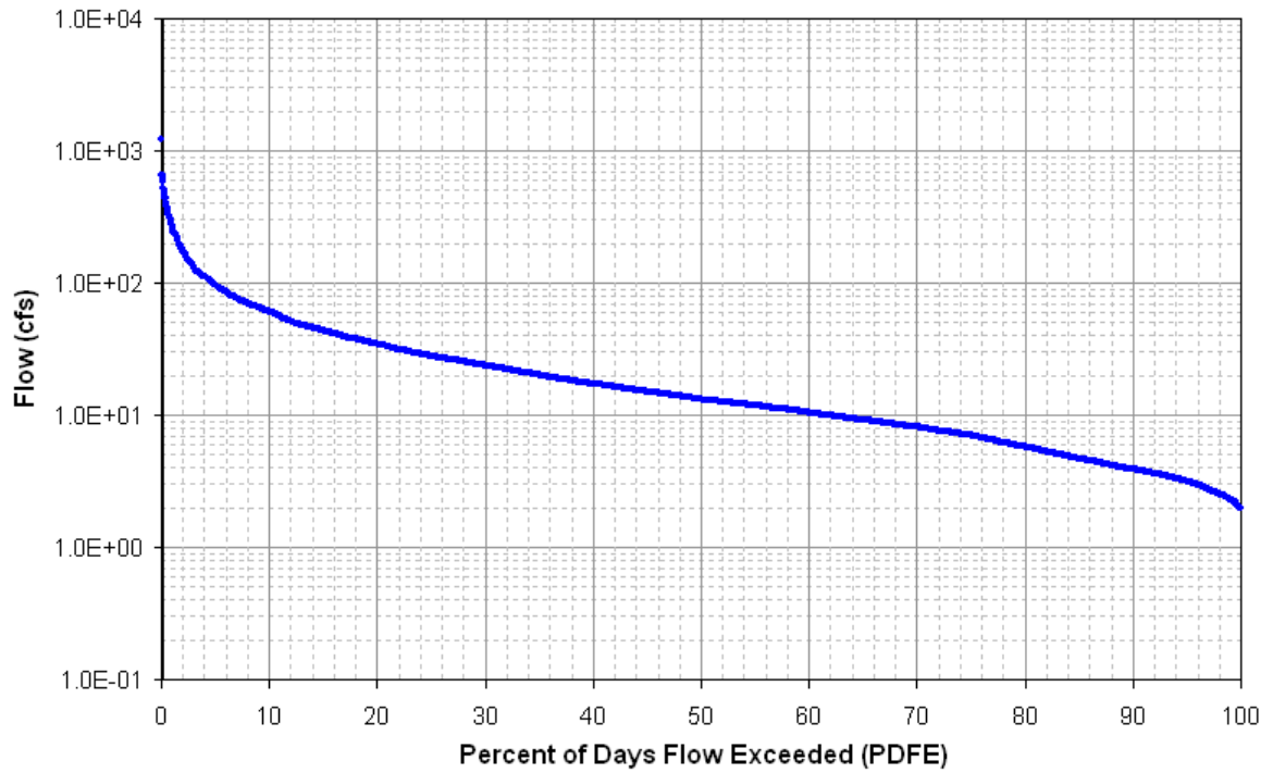
Figure E-1. Flow Duration Curve for Town Branch at Mile 0.1
