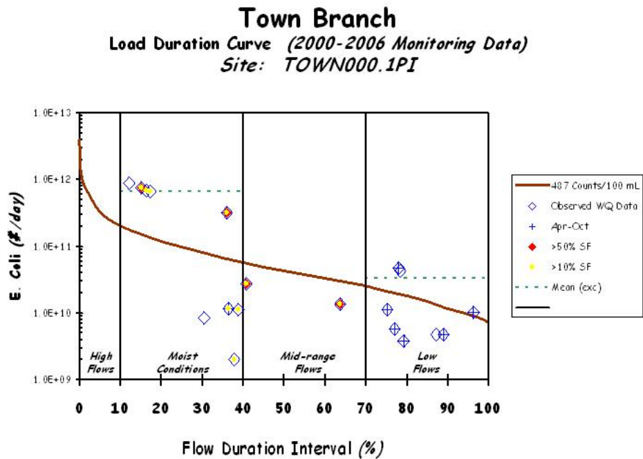
Figure C-2. E. Coli Load Duration Curve for Town Branch at Mile 0.1
