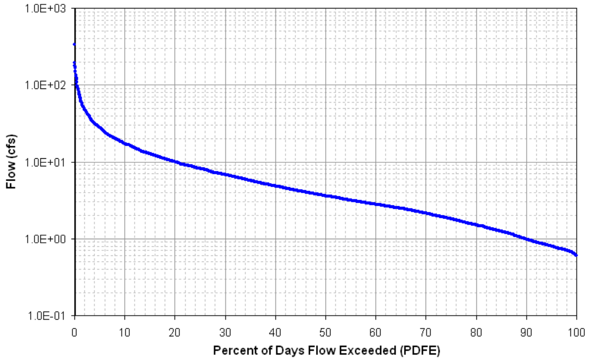
Figure C-1. Flow Duration Curve for Town Branch
