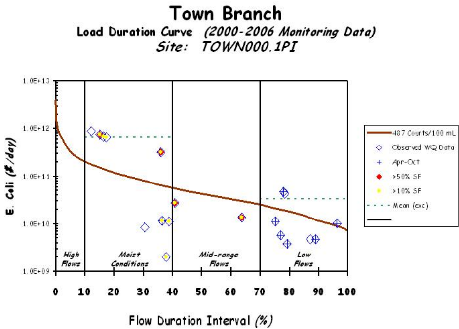
Figure E-2. E. Coli Load Duration Curve for Town Branch at Mile 0.1
