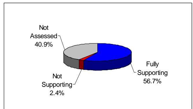
Water Quality Assessment of Streams and Rivers in the Tennessee Portion of the Clear Fork of the Cumberland River Watershed. Assessment data are based on the 2004 Water Quality Assessment of 442.6 stream miles in the watershed.
