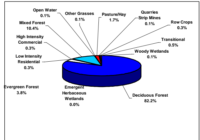
Land Use Distribution in the Tennessee Portion of the Clear Fork of the Cumberland River Watershed.
